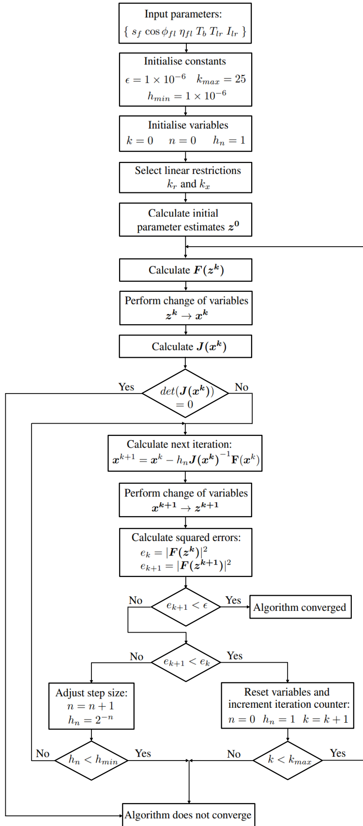
Figure 8: Flowchart for conventional NR algorithm
